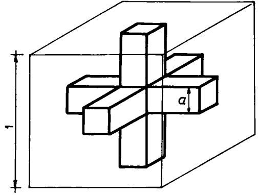
Figure 9 Unit volume of an ideal continuous porosity system.
