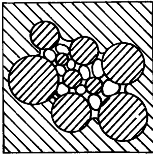
Figure 11 Schematic section of a concrete continuous porosity system of the bonded filler type.
