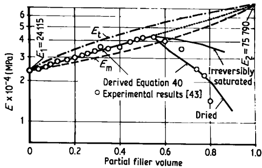
Figure 13 Hypothetical and measured values of the Young's modulus of cement mortar plotted against its composition.
